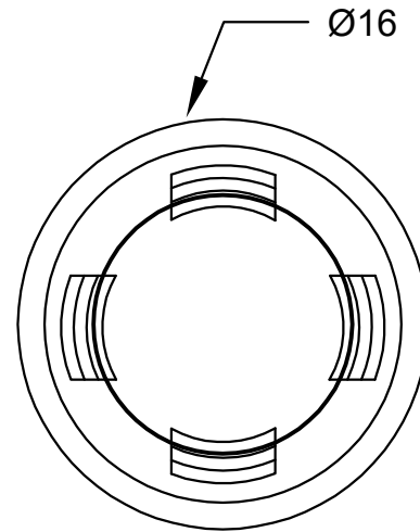
MOUNTING HOLE Ø12.0 THICKNESS 0.8-3.8
