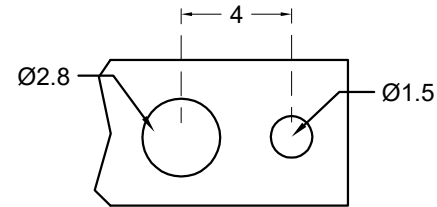
MOUNTING HOLE THICKNESS 1.7
