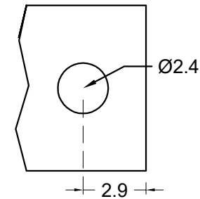
HOLE IN P.C.B THICKNESS : 1.3
